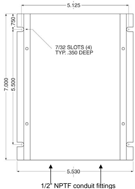
Diagram 7 Mounting Diagram
