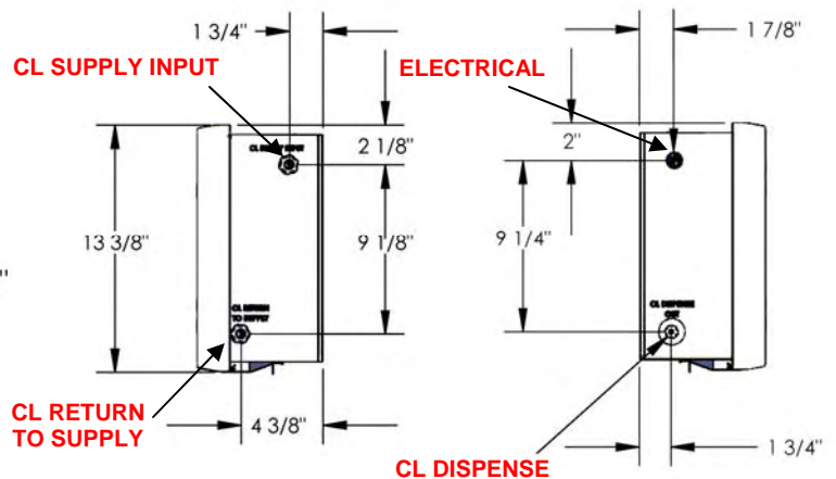
Diagram 2 (Right Side)
