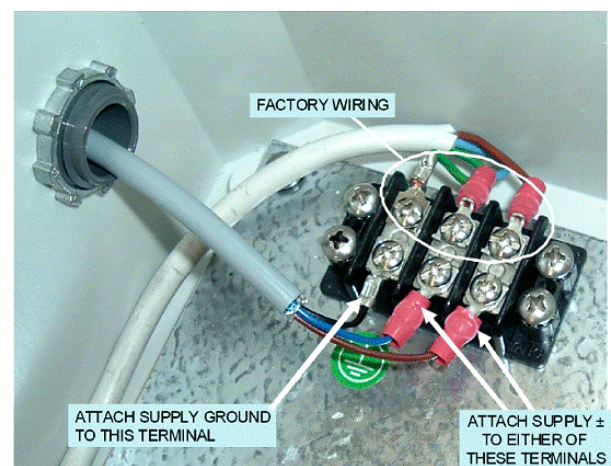
Diagram 4 Terminal Wiring
