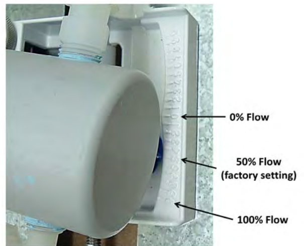
PUMP HEAD ANGLE (Displacement Adjustment)
