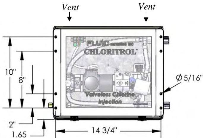
Diagram 1 Mounting Holes
